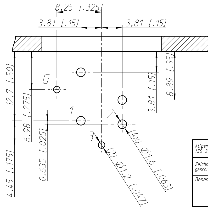
Layout tolerance: \pm 0,05 mm [0.002"]
