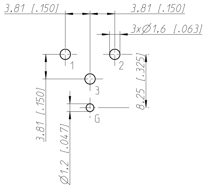
Layout tolerance: ±0.05mm [0.002"]
