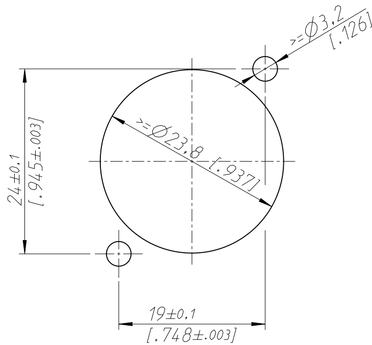
Panel cut out (rear side)
