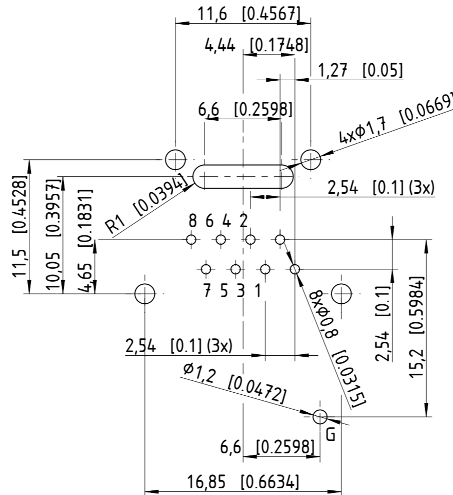
PCB- Layout (scale 3:1) = contact arrangement seen from backside (view to the very right)
